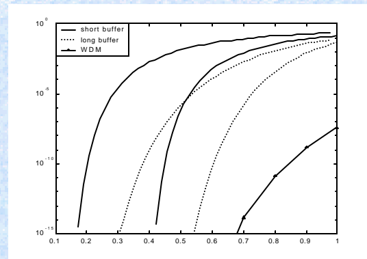
Comparison of packet loss/error probability
