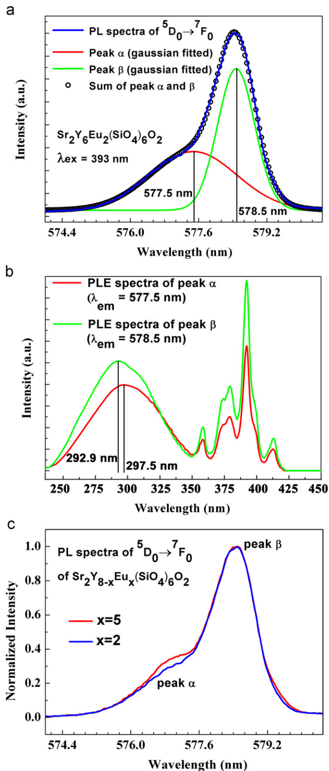
Fig. 7. (a) The high resolution PL spectra of the {}^5D_0 \rightarrow {}^7F_0 transition in \text{Sr}_2\text{Y}_6\text{Eu}_2(\text{SiO}_4)_6\text{O}_2 excited at 393 \text{ nm} . Double peak Gaussian fitting is performed and the peaks of \alpha and \beta are identified at 577.5 and 578.5 \text{ nm} . (b) The high resolution PLE spectra of peak \alpha and \beta . (c) The normalized high resolution PL spectra of the {}^5D_0 \rightarrow {}^7F_0 transitions in \text{Sr}_2\text{Y}_6\text{Eu}_2(\text{SiO}_4)_6\text{O}_2 and \text{Sr}_2\text{Y}_3\text{Eu}_5(\text{SiO}_4)_6\text{O}_2 . Both are excited at 393 \text{ nm} .
