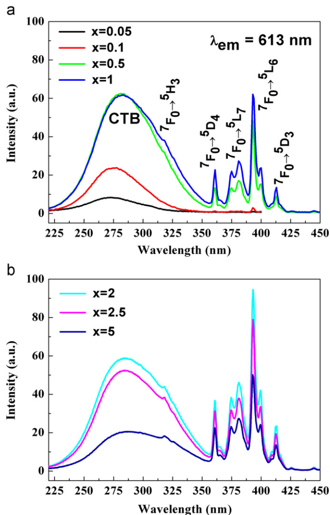
Fig. 5. The PLE spectra of \text{Sr}_2\text{Y}_{8-x}\text{Eu}_x(\text{SiO}_4)_6\text{O}_2 ( x=0.05, 0.1, 0.5, 1, 2.5, 5 ) with the emission wavelength fixed at 613 nm. The CTB and the intra- 4f transitions are indexed.
