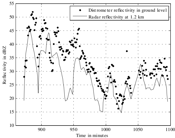
Figure 5. Time series inter-comparison between RADAR and distrometer reflectivity in dBZ for the rain event on 12th May 1998.
