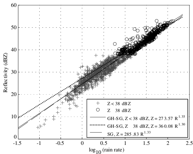
Figure 1. Scatter plot of reflectivity versus \log_{10} (rain rate) (1496 minutes of data from year 98 rain events, DSDs having rain drops greater than 100 only considered) and Z-R fits of SG and GH-SG.
