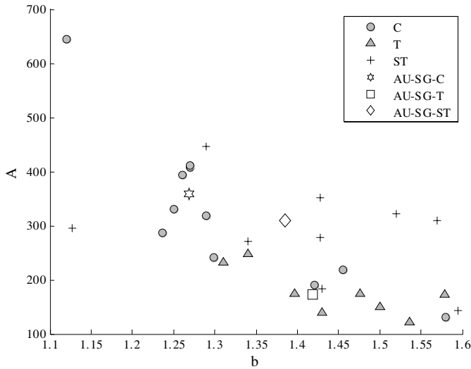
Figure 4. Relations between the coefficient A and the exponent b in the Z-R relations of the nine rain events for different rain types and for the AU-SG Z-R relation.
