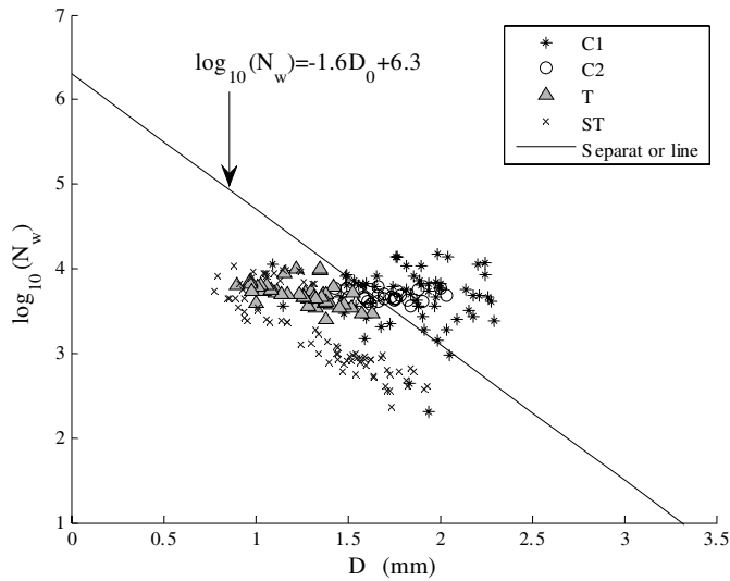
Figure 3. Dependence of \log_{10}(N_w) and D_0 (mm) for the rain event on 12th May 1998 where the unit of N_w is \text{mm}^{-1}\text{m}^{-3} . The separator line separates convective and stratiform points.
