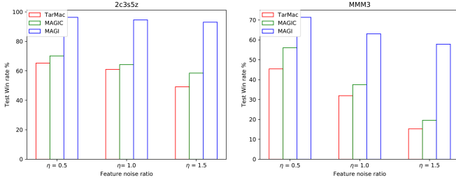
Fig. 6. Win rate with increasing feature noise ratio \eta .
