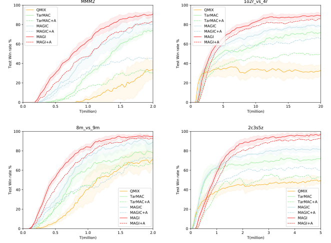
Fig. 4. Learning curves of different methods under adversarial attacks and noise ( \eta = 1.5 ).
