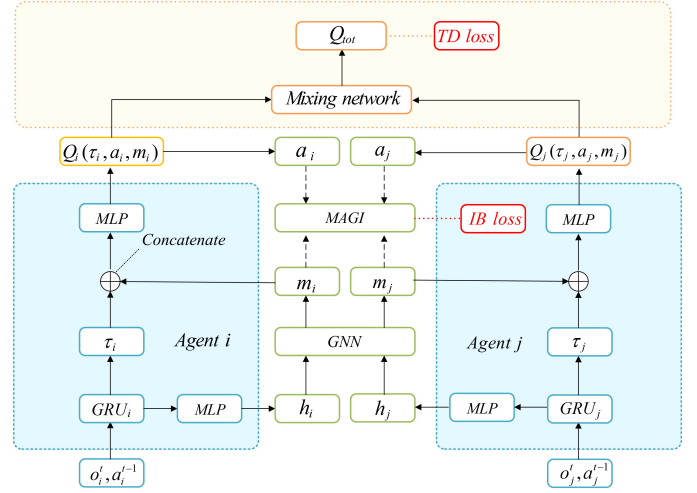
Fig. 2. The overall framework of MAGI.
