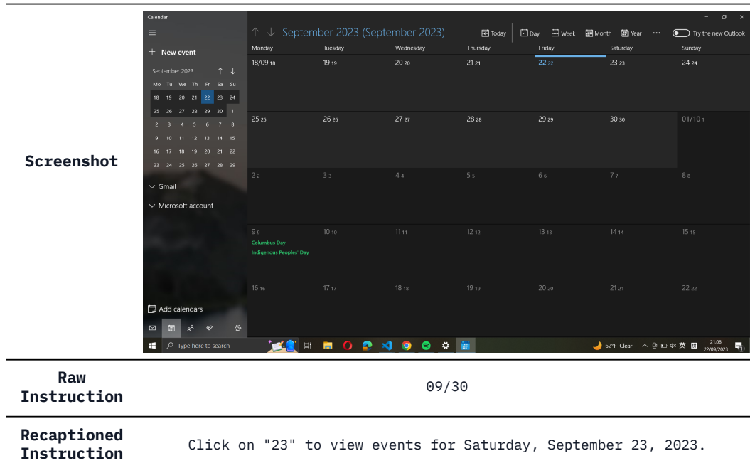
Figure 10: Example of incorrect instructions on desktop platforms sampled from OmniACT (Kapoor et al., 2024). The recaptioned instructions on GroundUI-1K are shown under the raw instructions from the original dataset.
