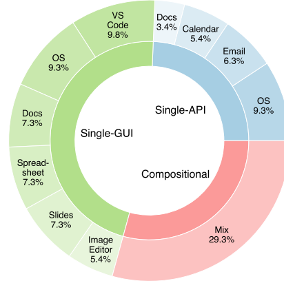
Figure 3: Task composition.
