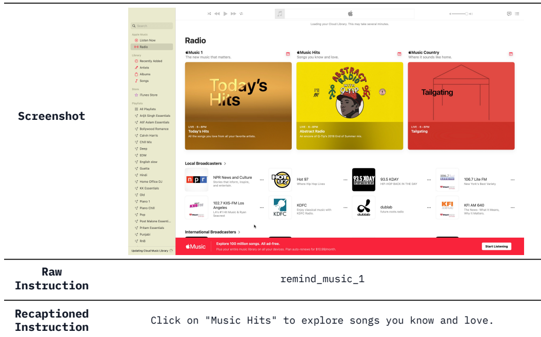
Figure 11: Example of ambiguous instructions on desktop platforms sampled from OmniACT (Kapoor et al., 2024). The recaptioned instructions on GroundUI-1K are shown under the raw instructions from the original dataset.
