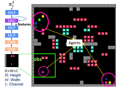
Figure 4: The green box to the lower left shows the agent's observation.
