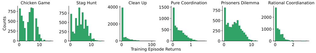
Figure 7: Histograms of training episode returns.
