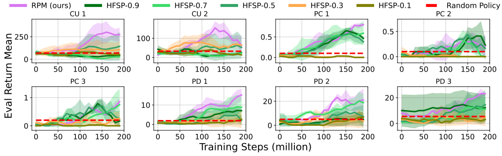
Figure 9: Ablation Studies: the results of HFSP with different sampling ratios.
