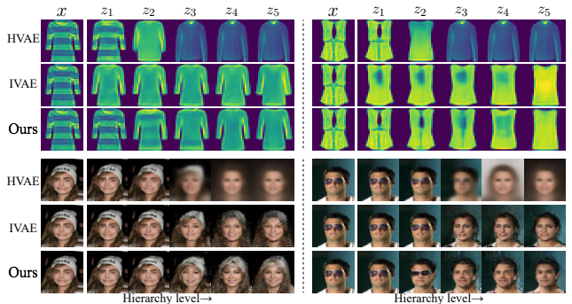
Figure 1. Visualization of different levels’ latent representations of hierarchical VAEs on FashionMNIST and CelebA [53] to demonstrate the learned hierarchical structure. HVAE fails to learn a 5-level hierarchy, where higher-level latent representations display posterior collapse , collapsing into the same modes of “clothing” and “female faces” regardless of the input. For IVAE, reconstructions of certain consecutive layers appear highly similar, suggesting a disrupted hierarchy. In contrast, our method preserves detailed information of inputs at low levels and captures increasingly abstract semantics at higher levels, mitigating posterior collapse and establishing an informative hierarchy.
