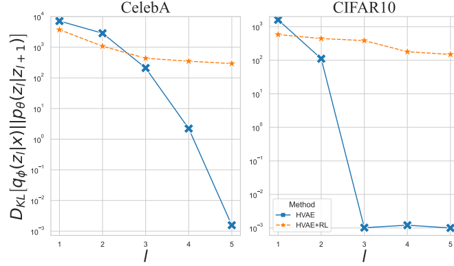
Figure 7. D_{KL}(q_\phi(z_l|x)||p_\theta(z_l|z_{l+1})) at different levels of hierarchical VAEs.
