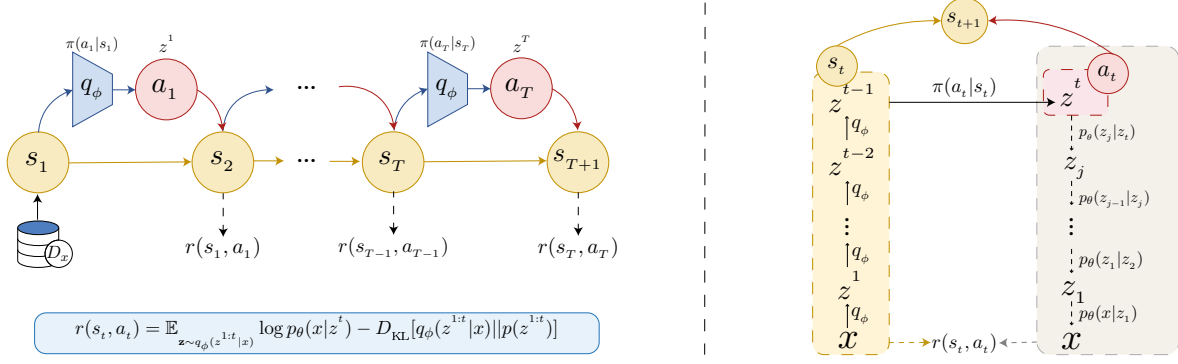
Figure 4. Illustration of modeling the inference process of a hierarchical VAE as a sequential decision process ( left ) and the details of the elements of RL s_t, a_t, s_{t+1} ( right ). A reward r(s_t, a_t) is derived with the skip-generative path depicted in the gray box.
