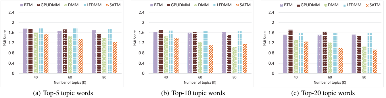
Figure 3: Topic Coherence on BaiduQA Dataset
