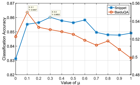
Figure 4: Effect of weight \mu under K = 40
