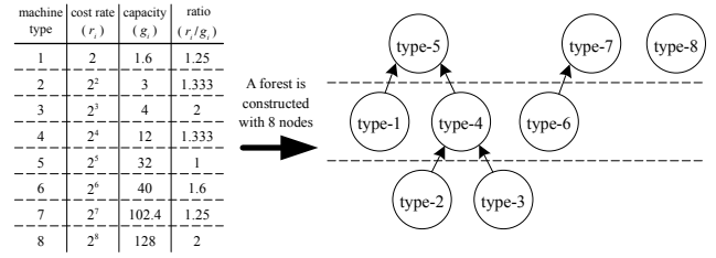
Fig. 2. Constructing a forest for the machine types
