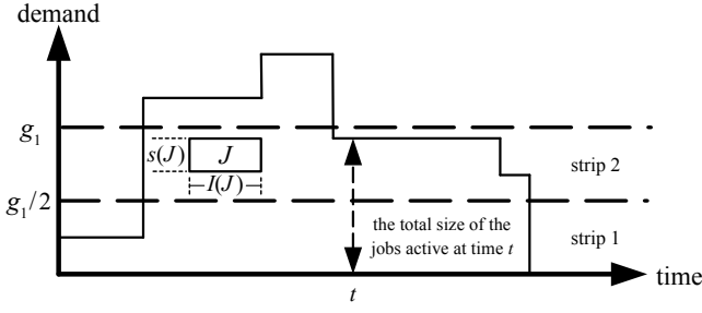
Fig. 1. Job placement in the demand chart
