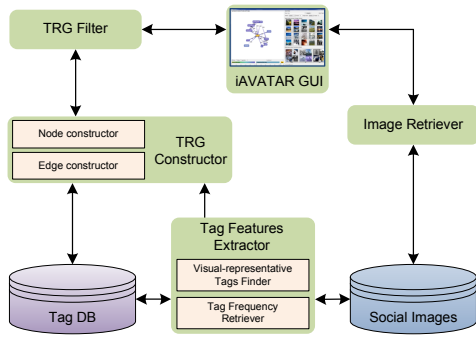
Figure 1: Architecture of iAVATAR .
