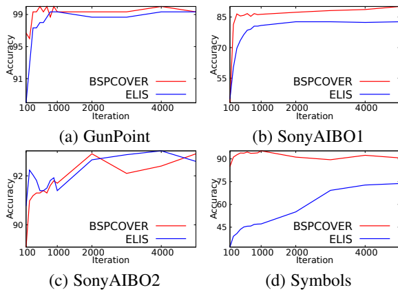
Fig. 11: Accuracy vs iterations of BSPCOVER and ELIS
