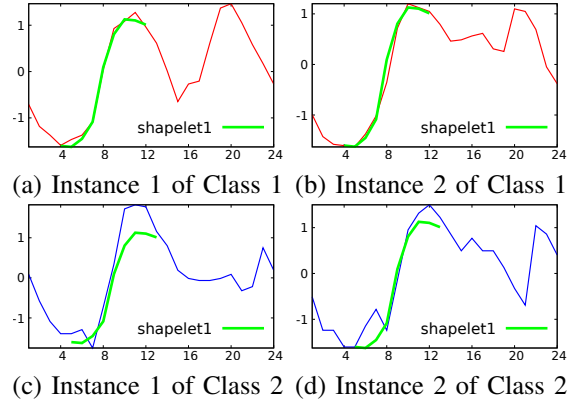
Fig. 3: A shapelet of ItalyPowerDemand highlighting the morning heating demand difference of summer and winter
