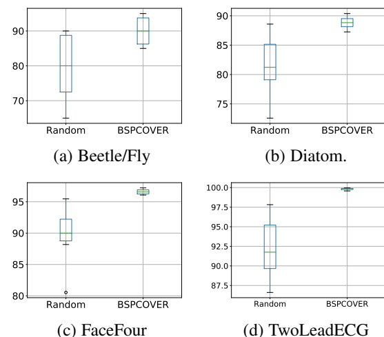
Fig. 9: Accuracy of Random vs BSPCOVER in box plots
