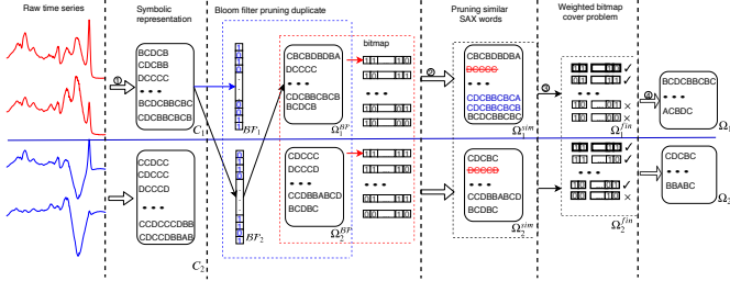
Fig. 2: An example of finding SAX words for model building
