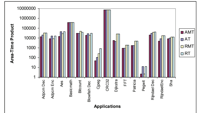
Fig. 3: Area-time product comparison between AMT , AT , RMT and RT
