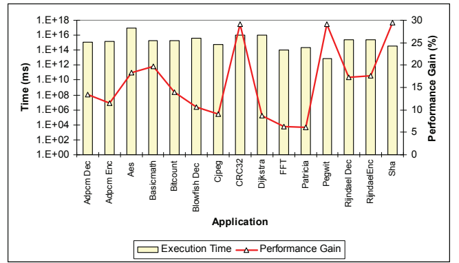
Fig. 6: Performance gain over base processor
