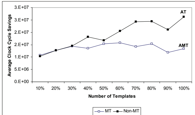
Fig. 4: Performance comparison with existing area optimization method
