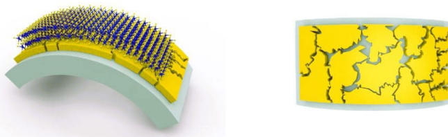
Left: illustration of the ultrathin layer of WS 2 integrated with gold nanostructures on the flexible substrate, which enables ultra-strong coupling between WS 2 excitons and gold plasmons. Right: Top view of the nanometre-sized gaps on the integrated surface, creating hotspots where ultra-strong coupling occurs. Credit: NTU.
