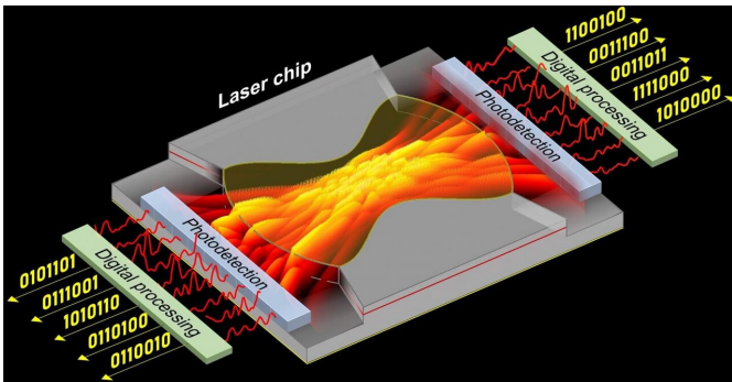
The NTU-designed system records light patterns caused by the reflection of a laser beam, which it then uses to generate a series of random numbers. Credit: NTU Singapore
