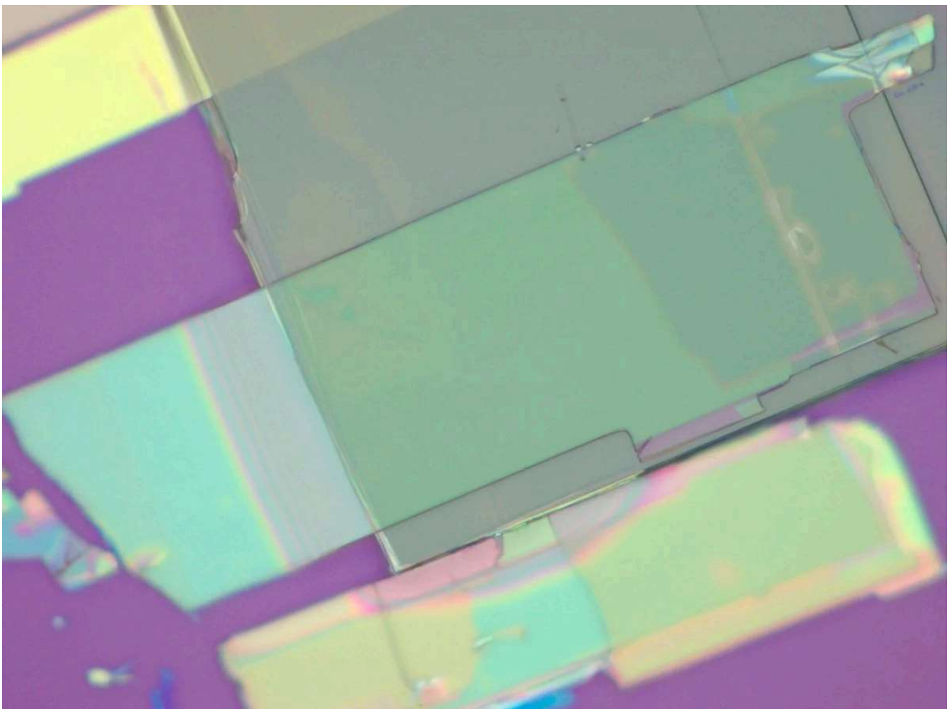
Two thin flakes of niobium oxide dichloride stacked on each other and photographed under a light microscope. One flake’s crystalline grain (grey flake) is positioned perpendicularly to the grain of the other flake (green flake). Credit:
