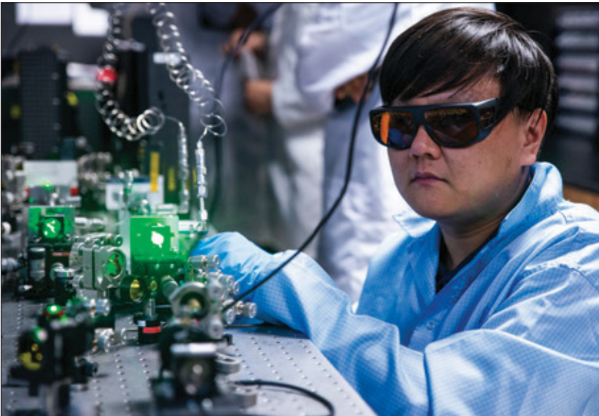
Research fellow Dr. Deng Ang from NTU Singapore's School of Electrical and Electronic Engineering calibrating the optical equipment in an experimental set-up with a green laser. The set-up is used to generate intense and ultra-fast mid-infrared lasers.
