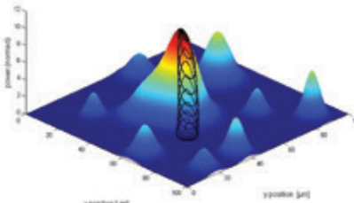
Fast Multi-Channel Gradient Search Algorithms
