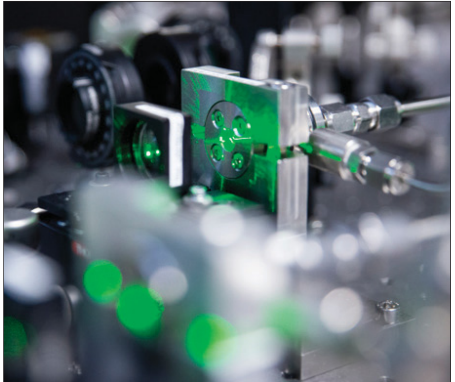
Image 4: The experimental set-up used to generate intense and ultra-fast mid-infrared lasers in NTU Singapore's study. A green laser is used to calibrate the set-up's optical equipment.
