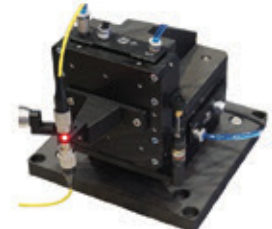
High-Speed Modular Air Bearing Alignment Systems for Wafer Probing
