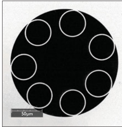
A scanning electron microscope photo of the cross-section of a hollow-core fiber used in NTU Singapore’s mid-infrared laser experiments. A ring of seven smaller tubes can be seen along the inner wall of the fiber core.
