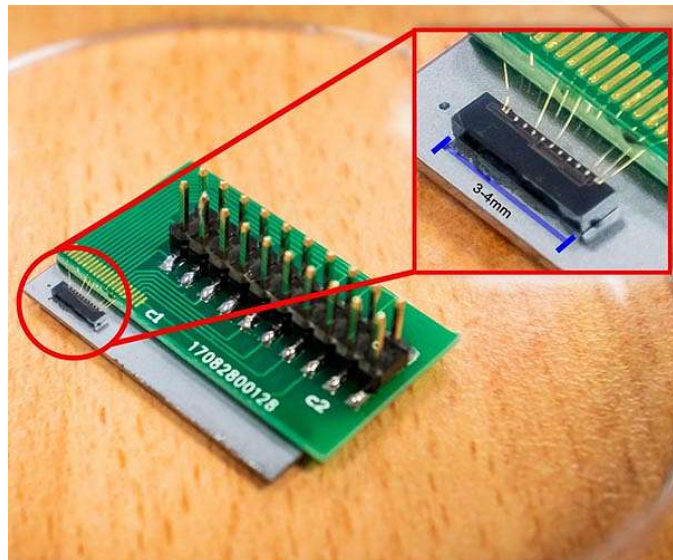
Roughly about 3mm in size, tiny chip developed by NTU scientists uses quantum communication algorithms to provide enhanced security compared to existing industry standards. It also needs 1,000 times less space than current quantum communication setups, opening doors for more secure communication technologies that can be deployed in compact devices such as smartphones, tablets and smart watches.
