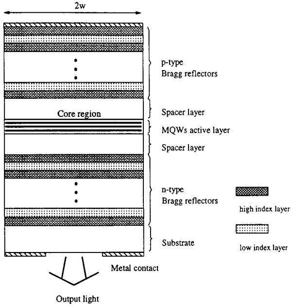
Fig. 2. Schematic of an index-guided VCSEL.
