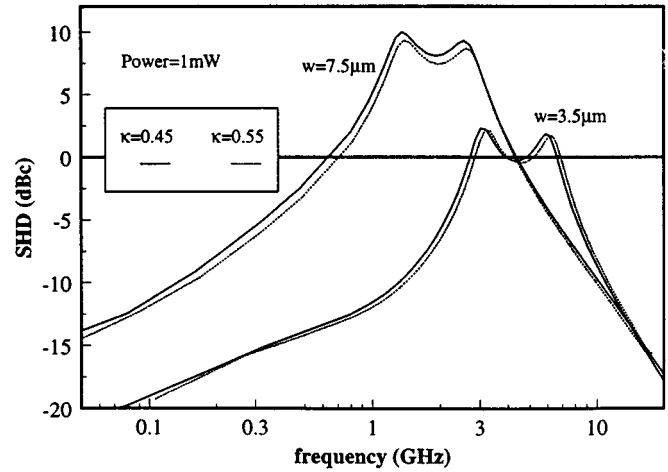
Fig. 12. Second harmonic distortion of VCSEL's with core radius of 3.5 and 7.5 \mu\text{m} under the influence of \kappa . The steady state output power of lasers is 1 mW. Solid lines: \kappa = 0.45 \text{ Wcm}^{-1} \text{ C}^{-1} ; and dotted lines: \kappa = 0.55 \text{ Wcm}^{-1} \text{ C}^{-1} .
