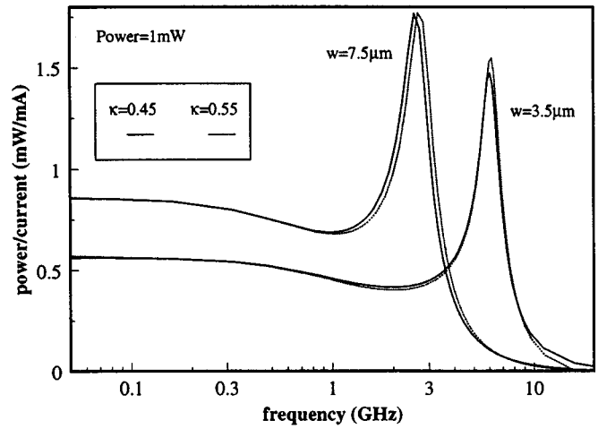
Fig. 11. Amplitude modulation response of VCSEL's with core radii of 3.5 and 7.5 \mu\text{m} under the influence of \kappa . The steady-state output power of the lasers is 1 mW. Solid lines: \kappa = 0.45 \text{ Wcm}^{-1} \text{ C}^{-1} ; and dotted lines: \kappa = 0.55 \text{ Wcm}^{-1} \text{ C}^{-1} .
