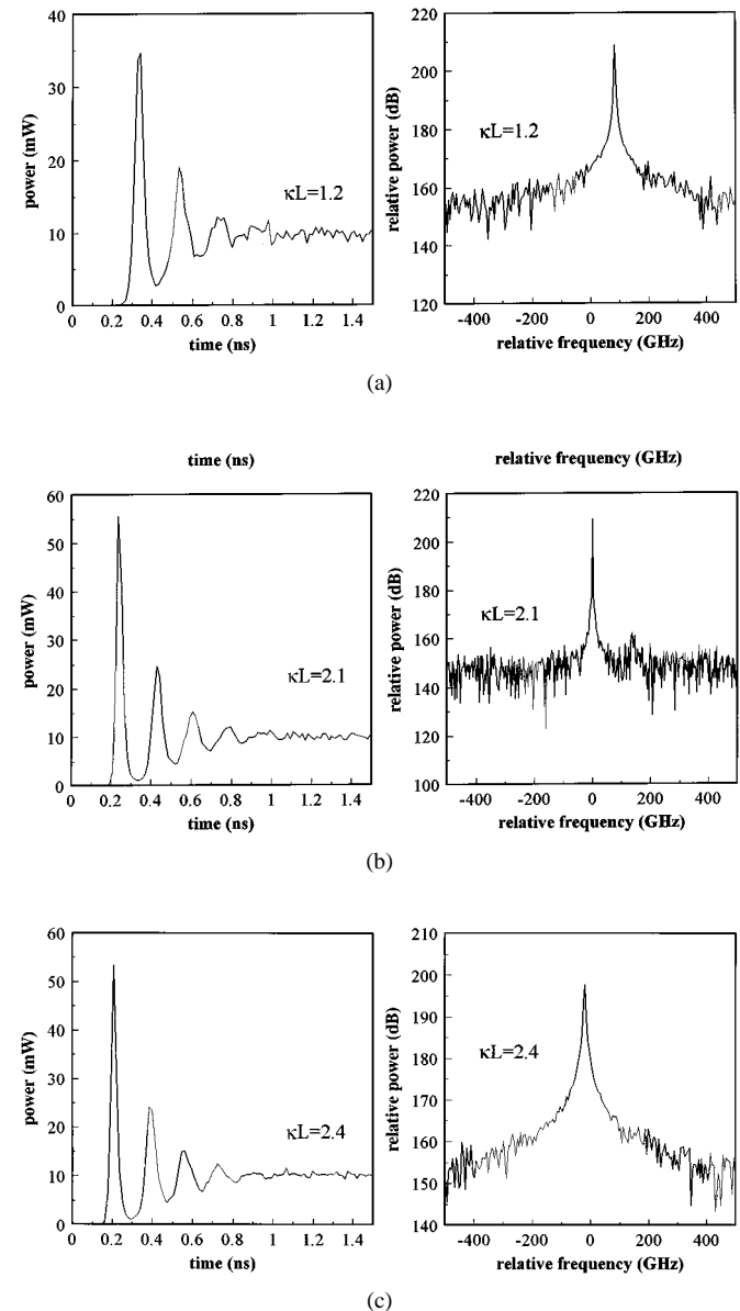
Fig. 11. The transient optical power response and steady-state spectra of DFB laser with double tapered waveguide structure. (a) \kappa L = 1.2 , (b) \kappa L = 2.1 , and (c) \kappa L = 2.4 .
