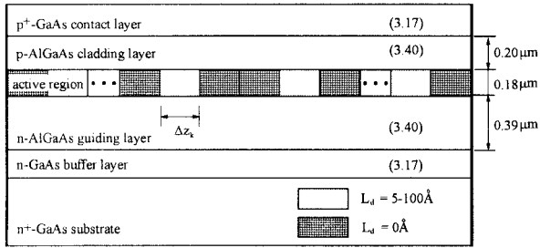
Fig. 15. Schematic diagram of a FP laser with periodic diffused QW structure.
