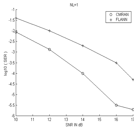
Fig. 4 SER performance, NL=1
