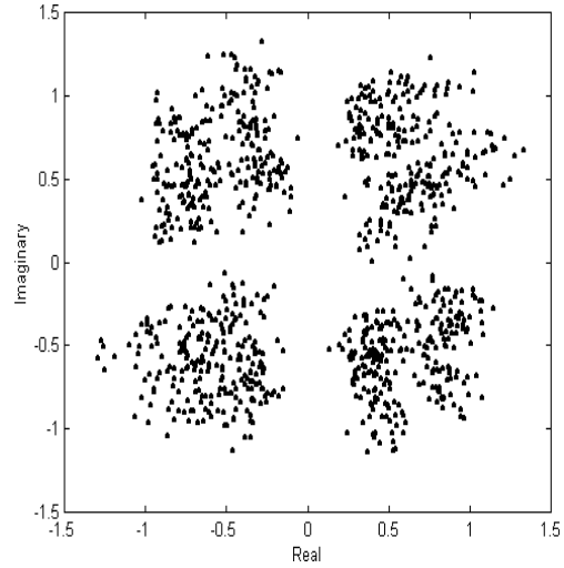
Fig 13. CRBF/SG equalizer output (after 14000 training iterations)
