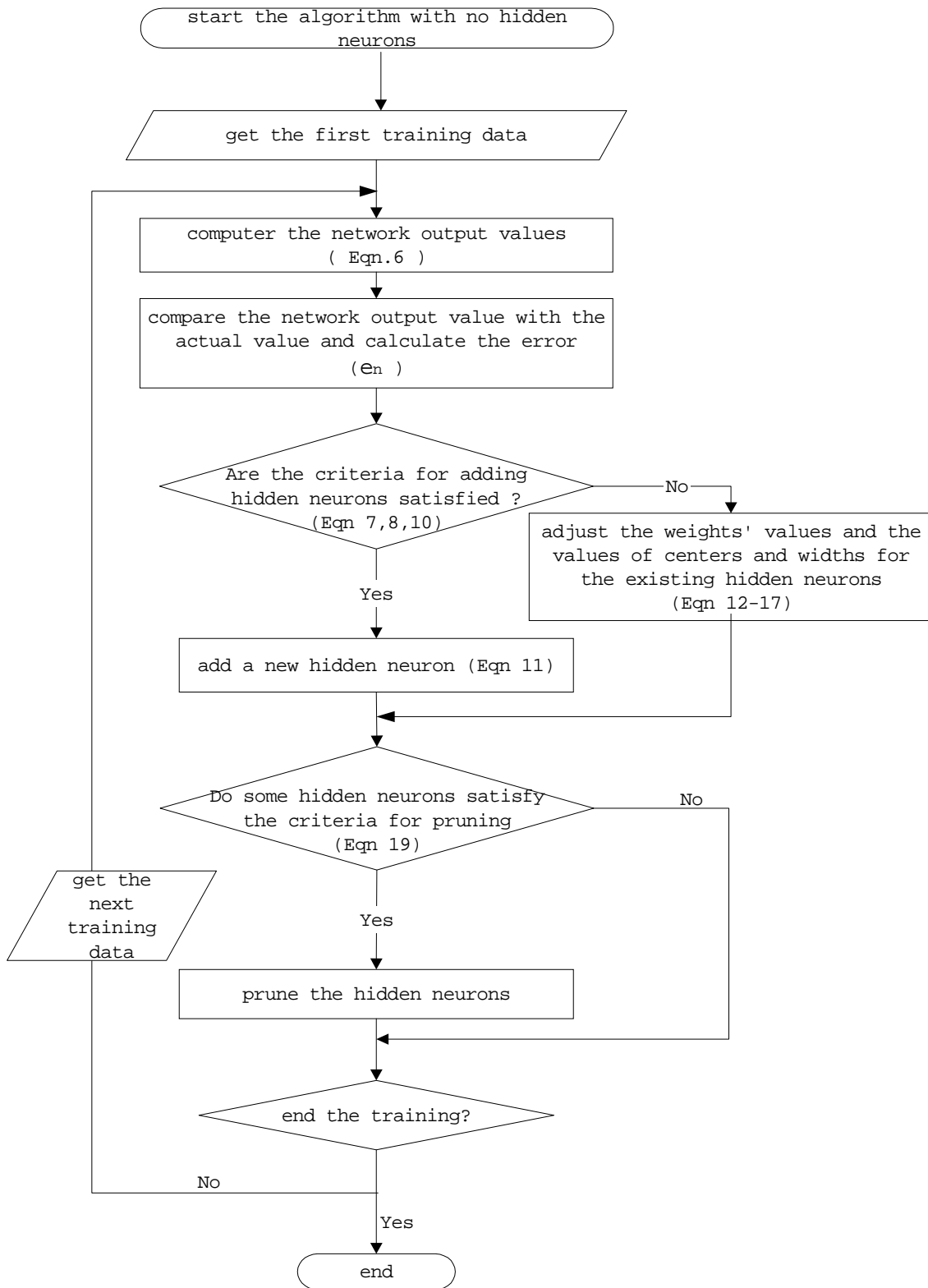
Fig.2 Flow diagram for CMRAN learning Algorithm
