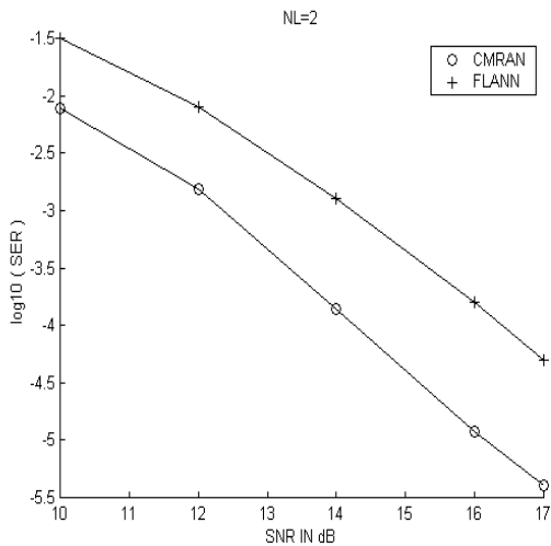
Fig. 5 SER performance, NL=2
