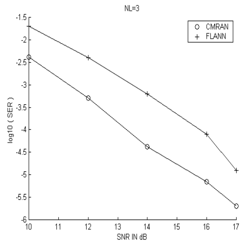
Fig. 6 SER performance, NL=3
