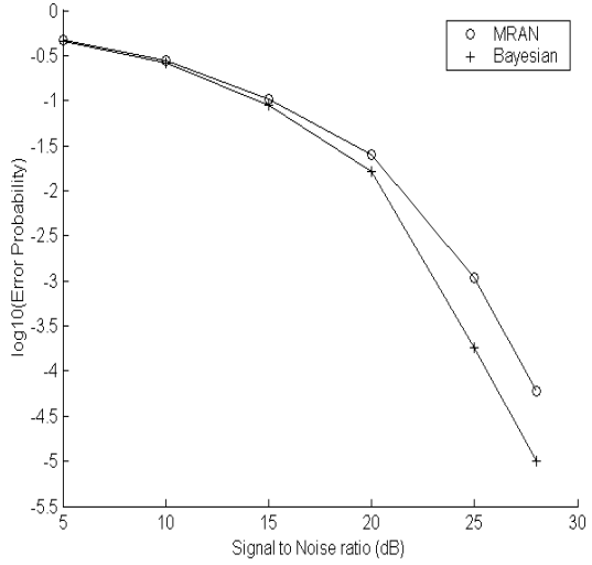
Fig.10 Error curves for CMRAN and Bayesian equalizer
