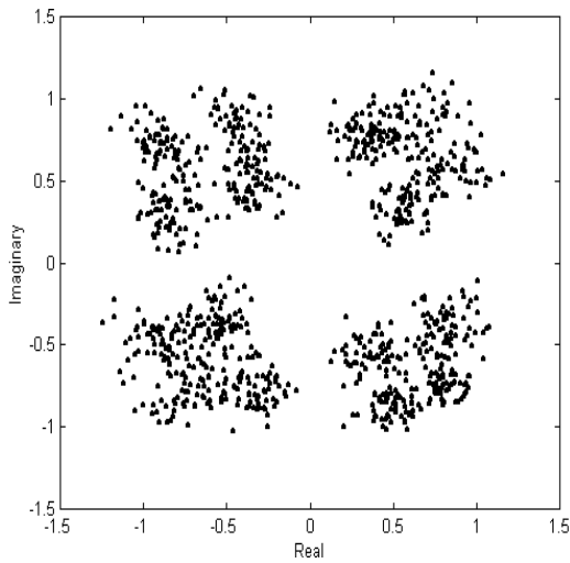
Fig 12. CMRAN equalizer output (after 4000 training iterations)
