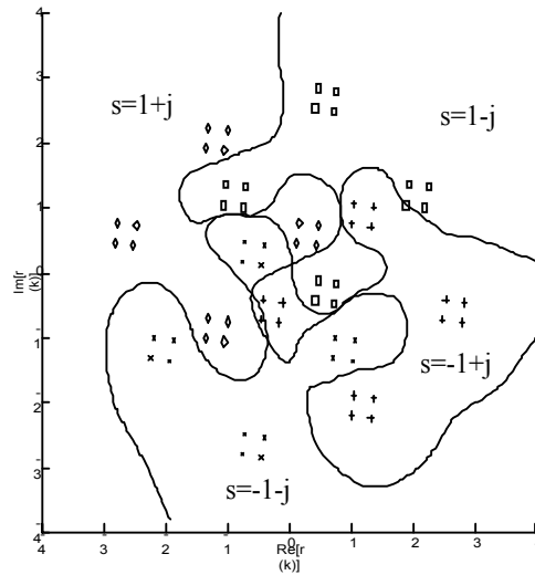
Fig.8 Complex MRAN boundary (with 52 neurons)
