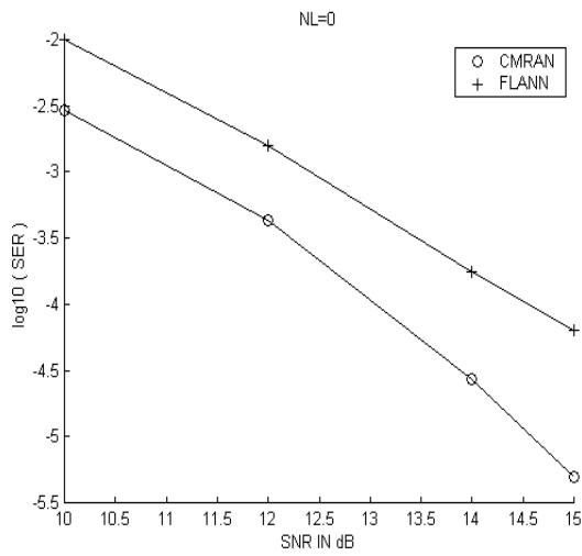
Fig. 3 SER performance, NL=0
