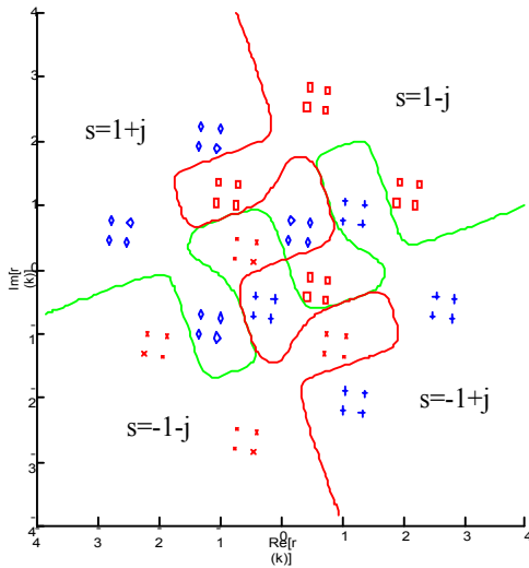
Fig. 7 Bayesian boundary (with 64 states)
