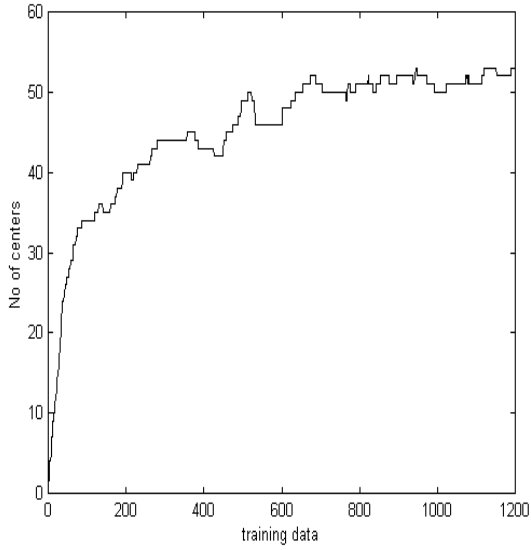
Fig.9 Growth of hidden neurons as training processes
