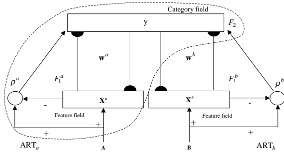
Figure 2: The Adaptive Resonance Associative Map architecture
