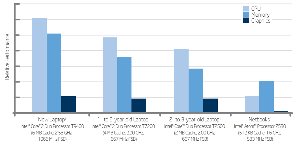
Figure 1. Laptops were much faster than netbooks for processor- or graphics-intensive applications. Intel internal measurements, March 2009.
